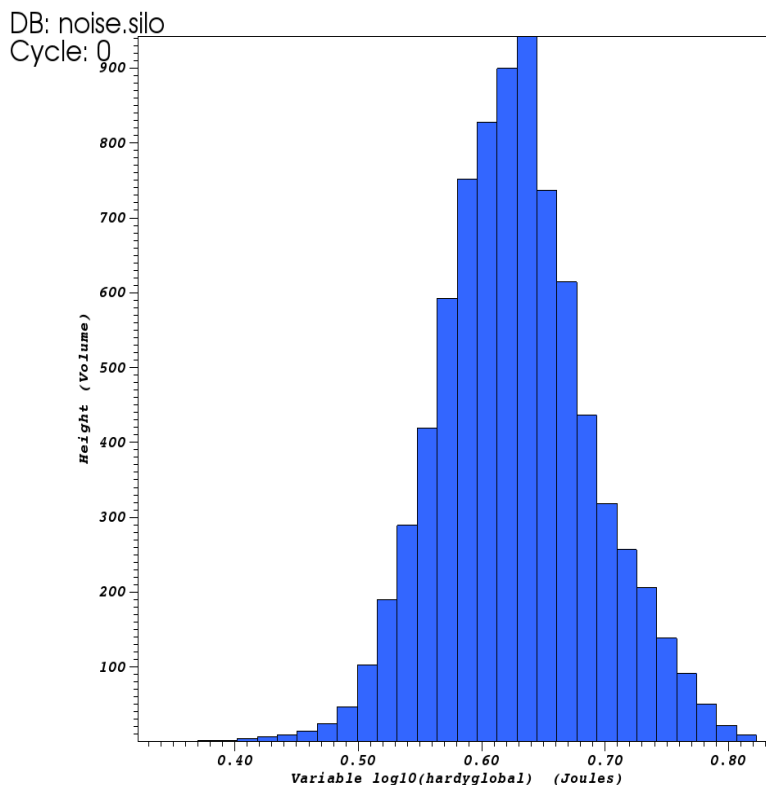
Fig. 3.40: Histogram plot
