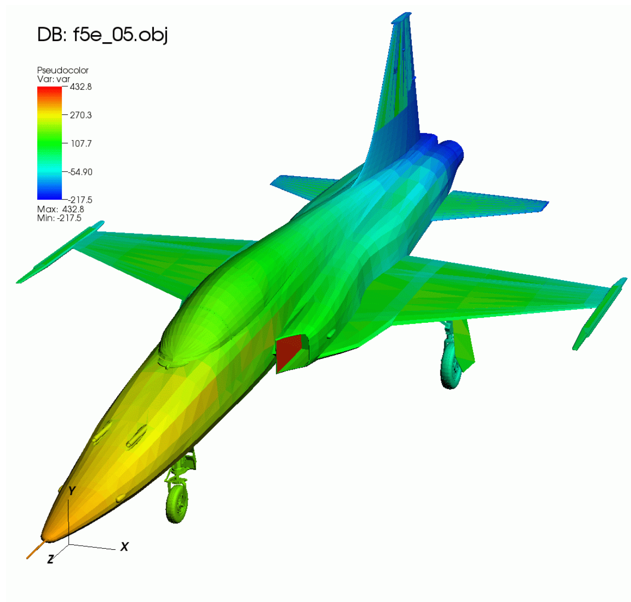
Fig. 3.56: Pseudocolor plot
