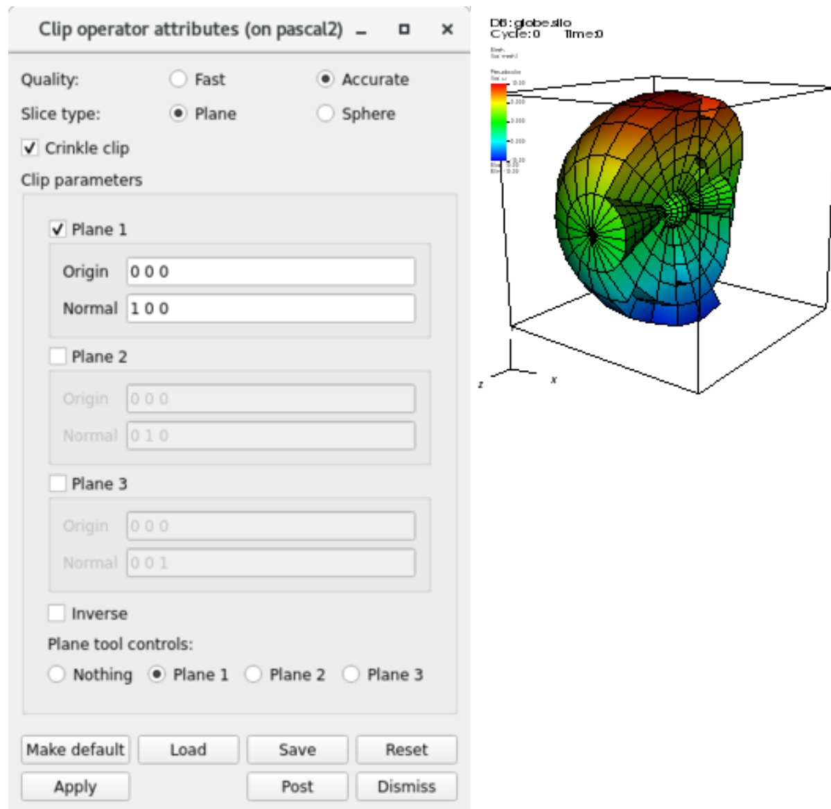
Fig. 3.95: Enabling the Crinkle clip option; Crinkle clip example
