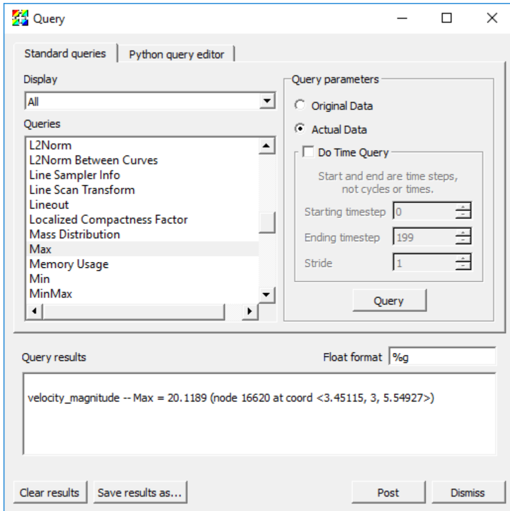
Fig. 5.43: The result of the velocity magnitude query.
