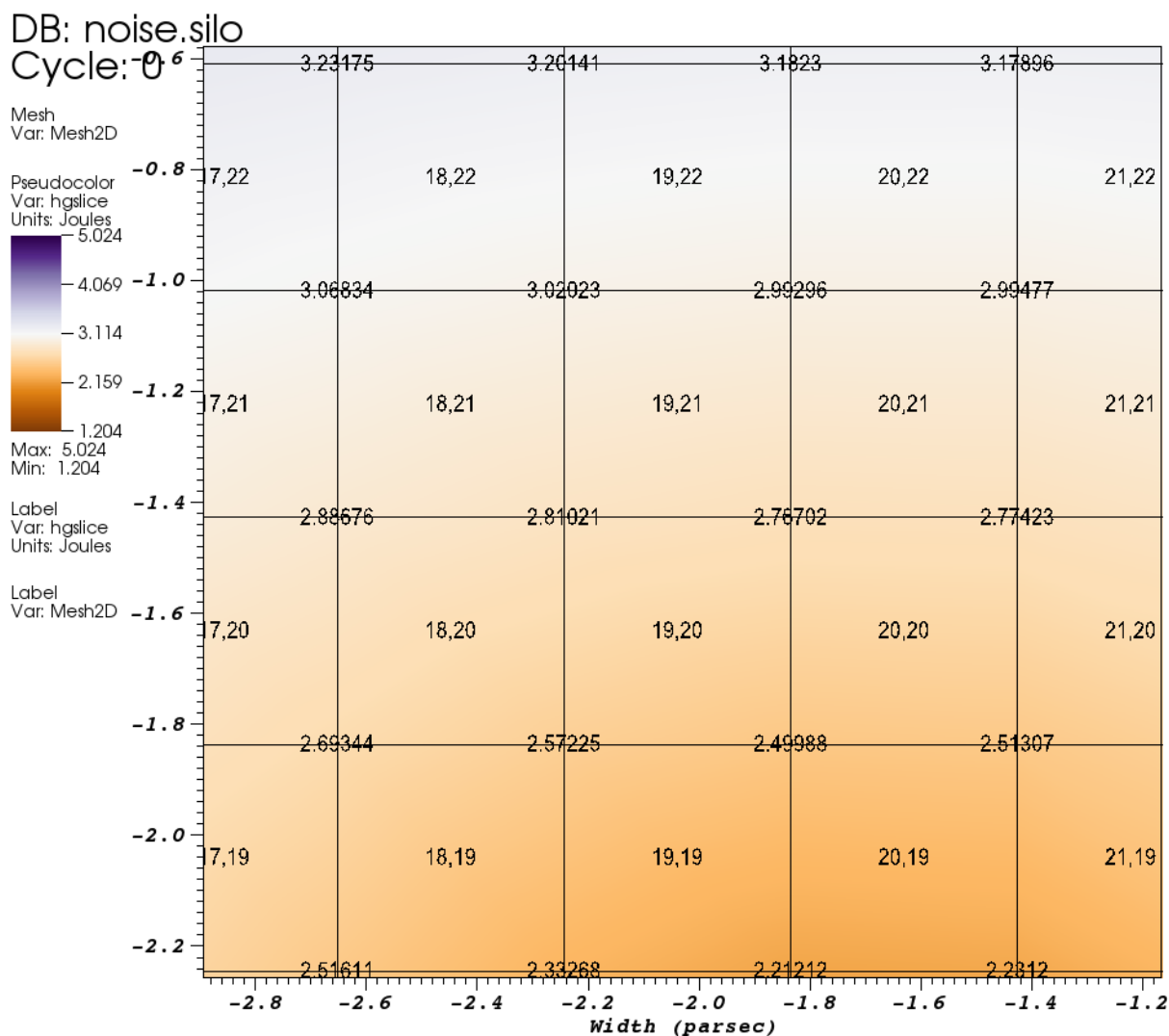
Fig. 3.42: Label plot of the mesh overlayed on Pseudocolor and Mesh plots
