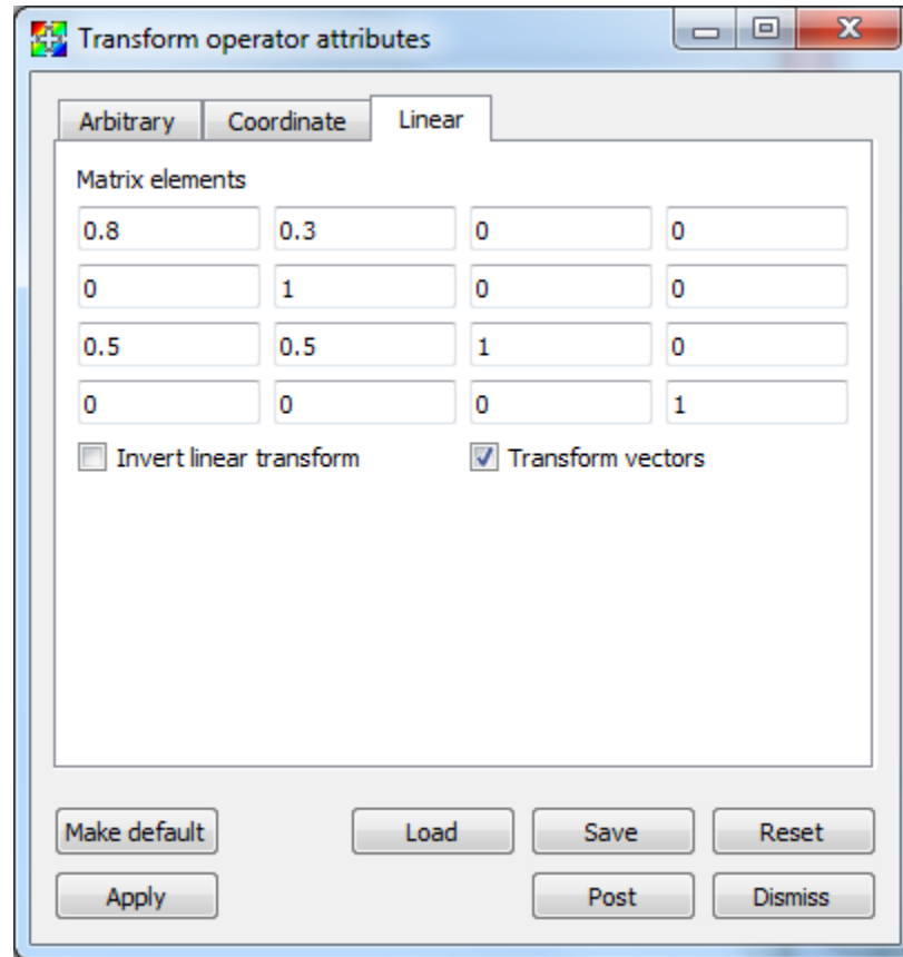
Fig. 3.157: Linear transformation options
