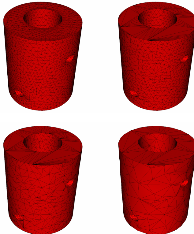
Fig. 3.104: Decimate operator applied to reduce the number of cells in the mesh. (Left-to-right, top-to-bottom): Original Mesh, Reduction = 0.1, Reduction = 0.5, Reduction = 0.75
