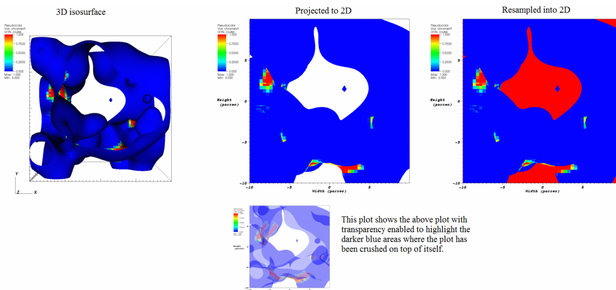
Fig. 3.135: Using the Resample operator to create a 2D projection
