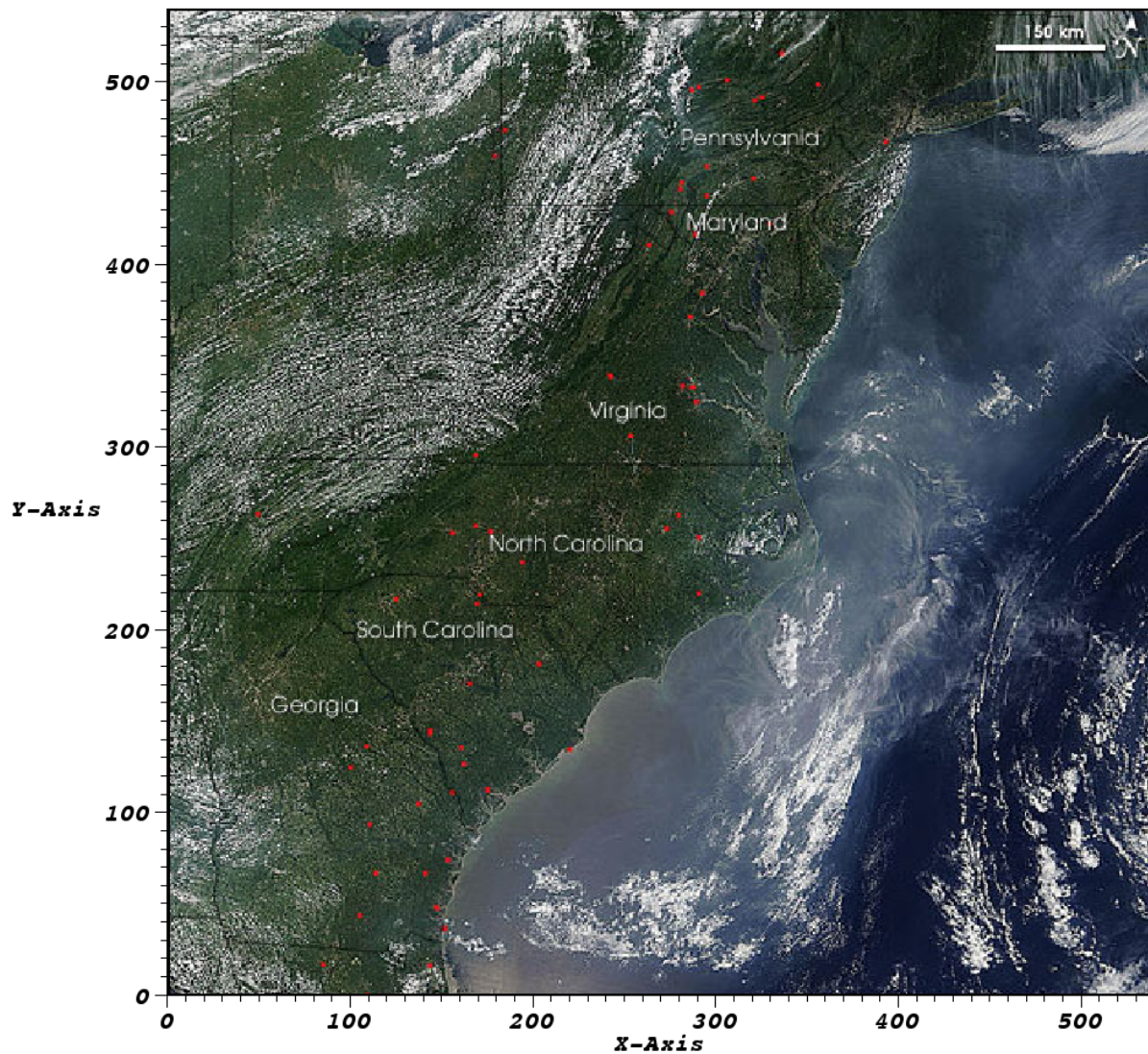
Fig. 3.68: Truecolor Plot
