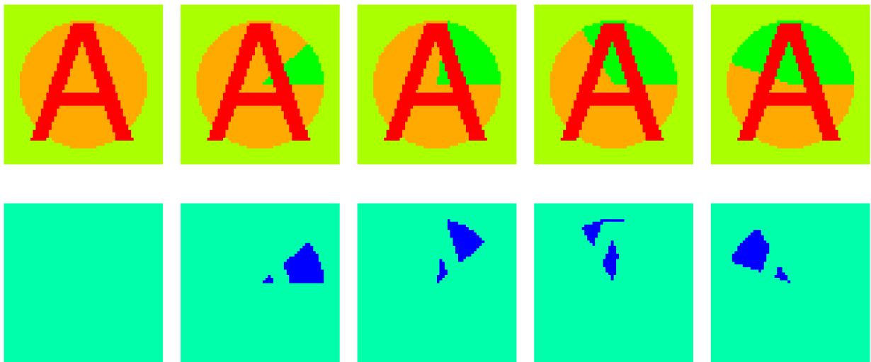
Fig. 3.343: Plot of a variable and its time derivative plot
