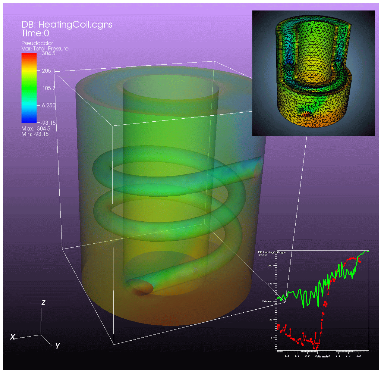
Fig. 3.283: An Example of a visualization with two overlaid image annotations
