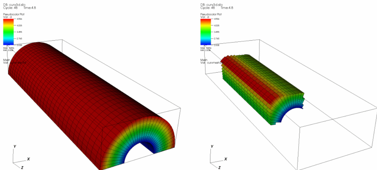
Fig. 3.90: Box operator example (original on left, with Box operator applied on right)
