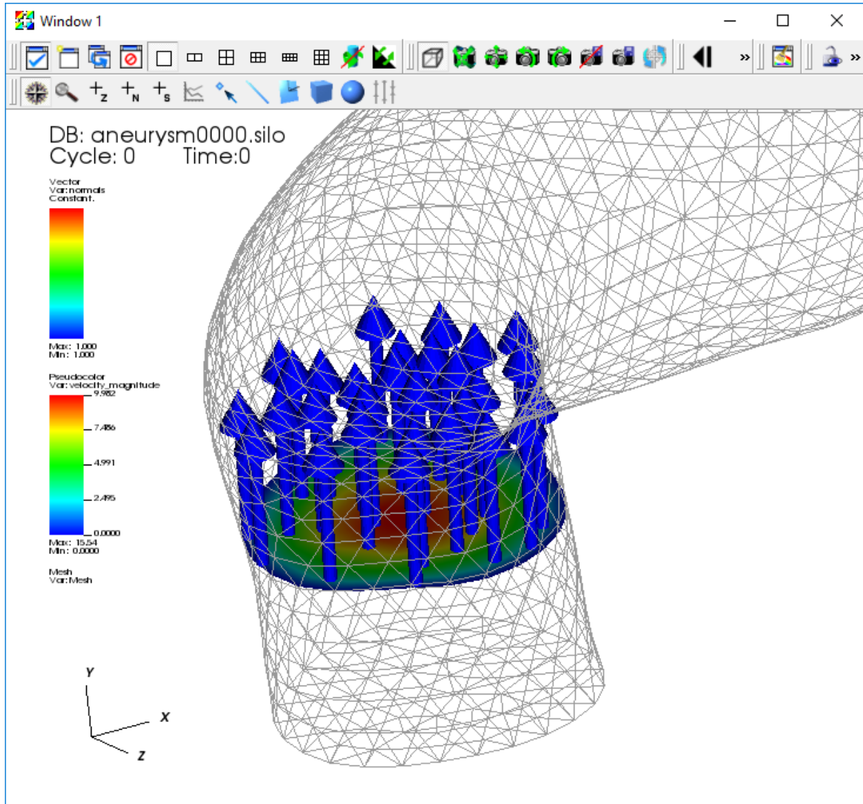
Fig. 5.56: The Vector plot of the normals.
