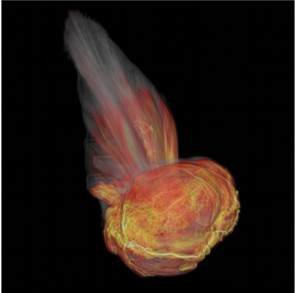
Fig. 3.71: Type Ia Supernova (Image Credit: Blue Waters visualization staff, Rob Sisneros and Dave Semeraro)
