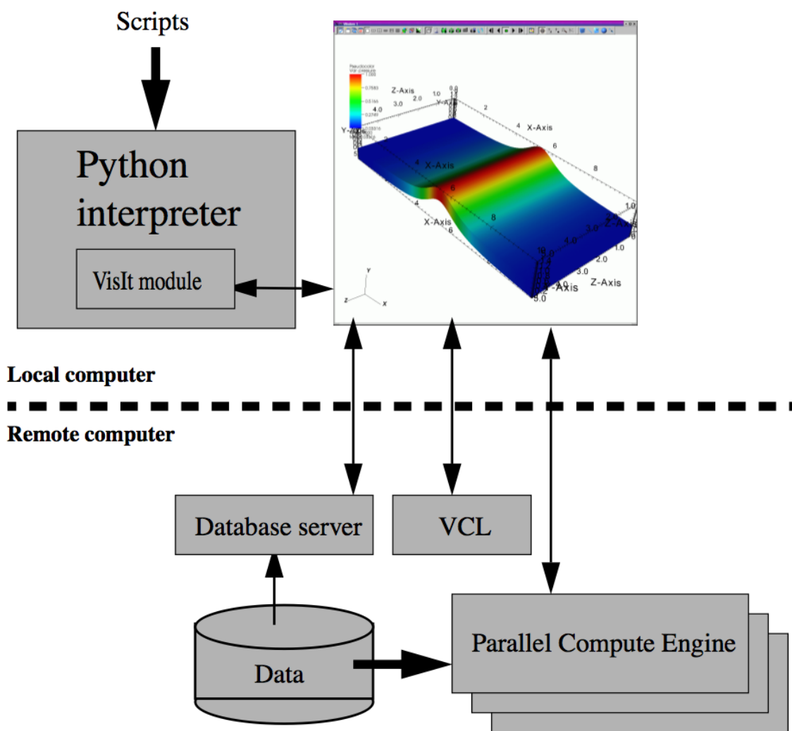
Fig. 4.1: VisIt's architecture
