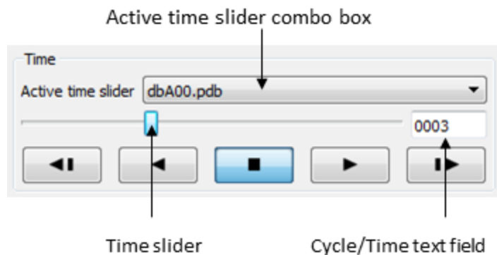
Fig. 1.282: Time slider and related controls
