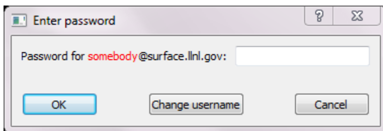
Fig. 1.302: Password Window
