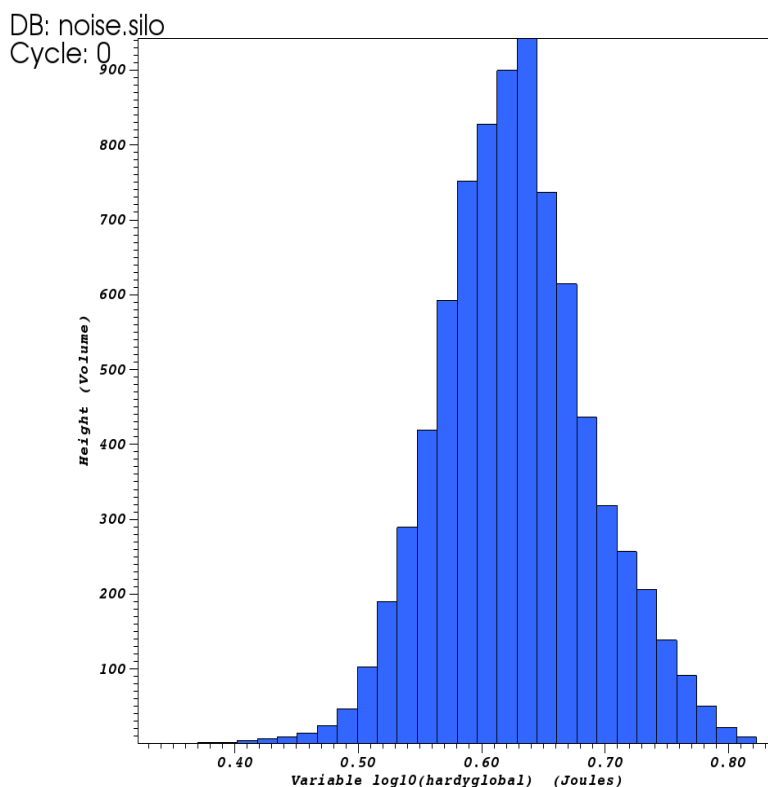
Fig. 1.40: Histogram plot
