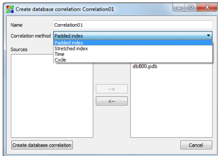
Fig. 1.291: Correlation methods
