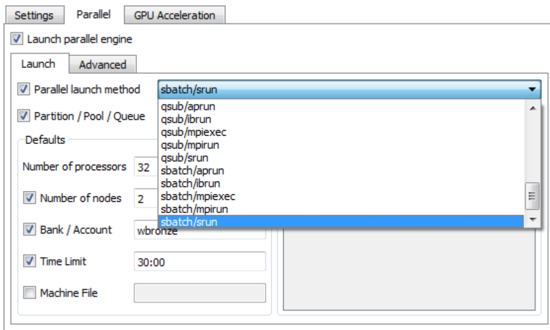
Fig. 1.309: Parallel launch method options
