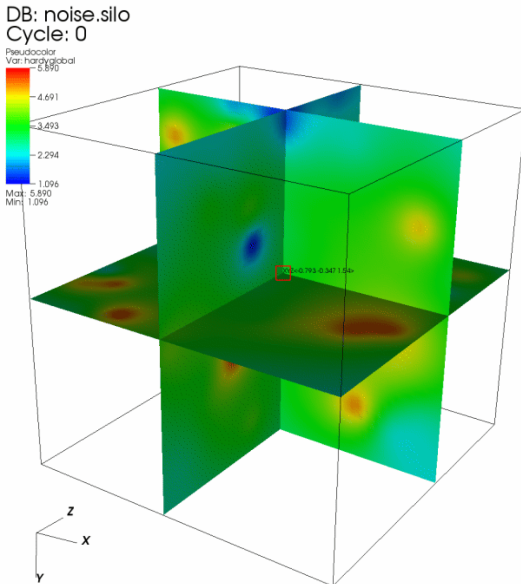
Fig. 1.278: Point tool
