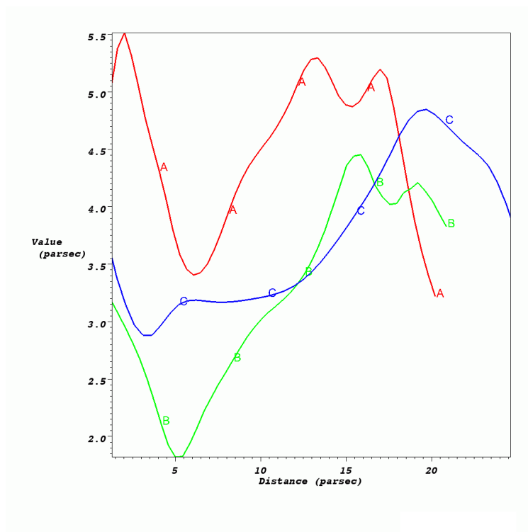
Fig. 1.33: Curve plot
