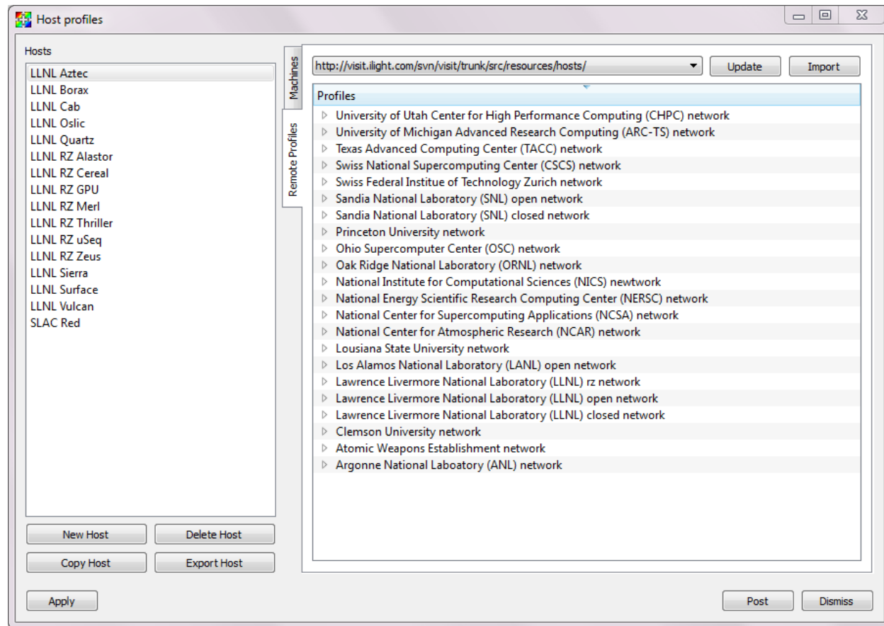
Fig. 1.317: Remote Profiles tab with updated content
