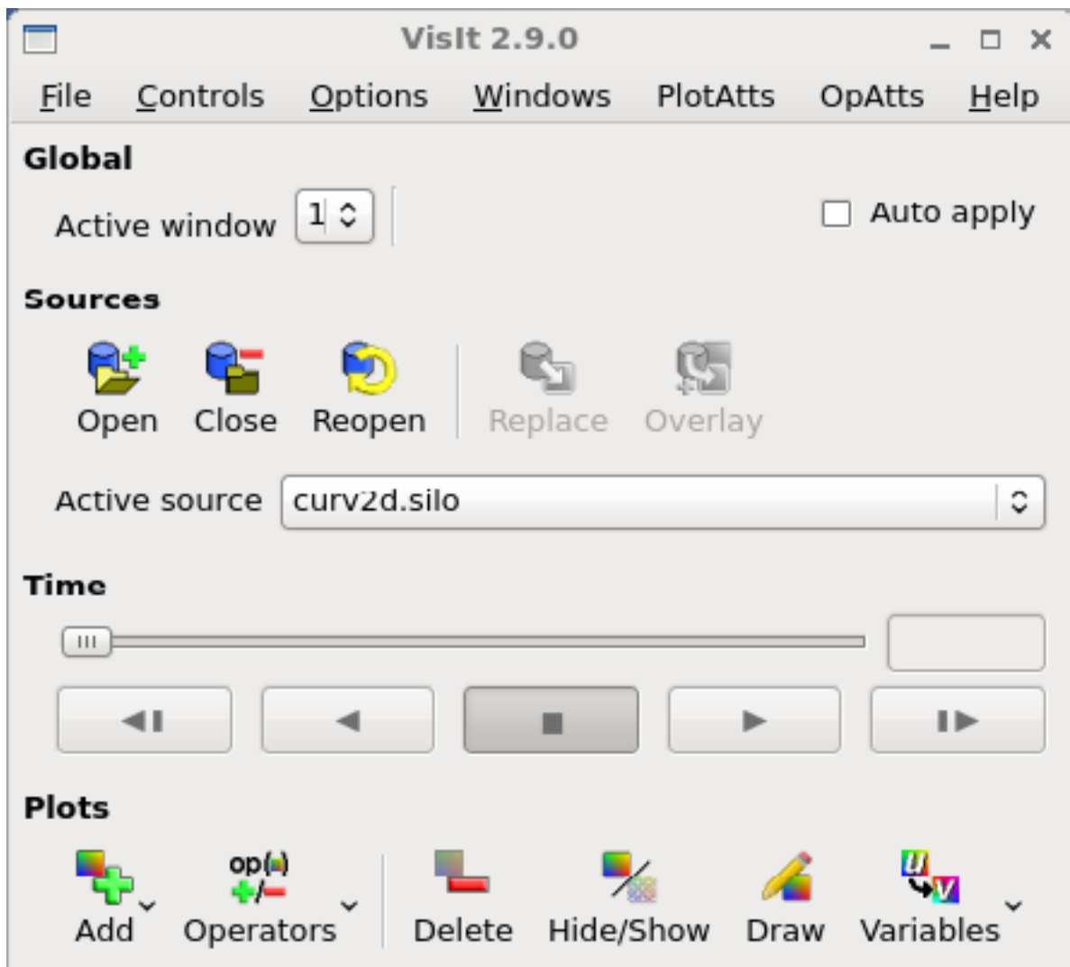
Fig. 1.9: Main gui panel showing Sources section
