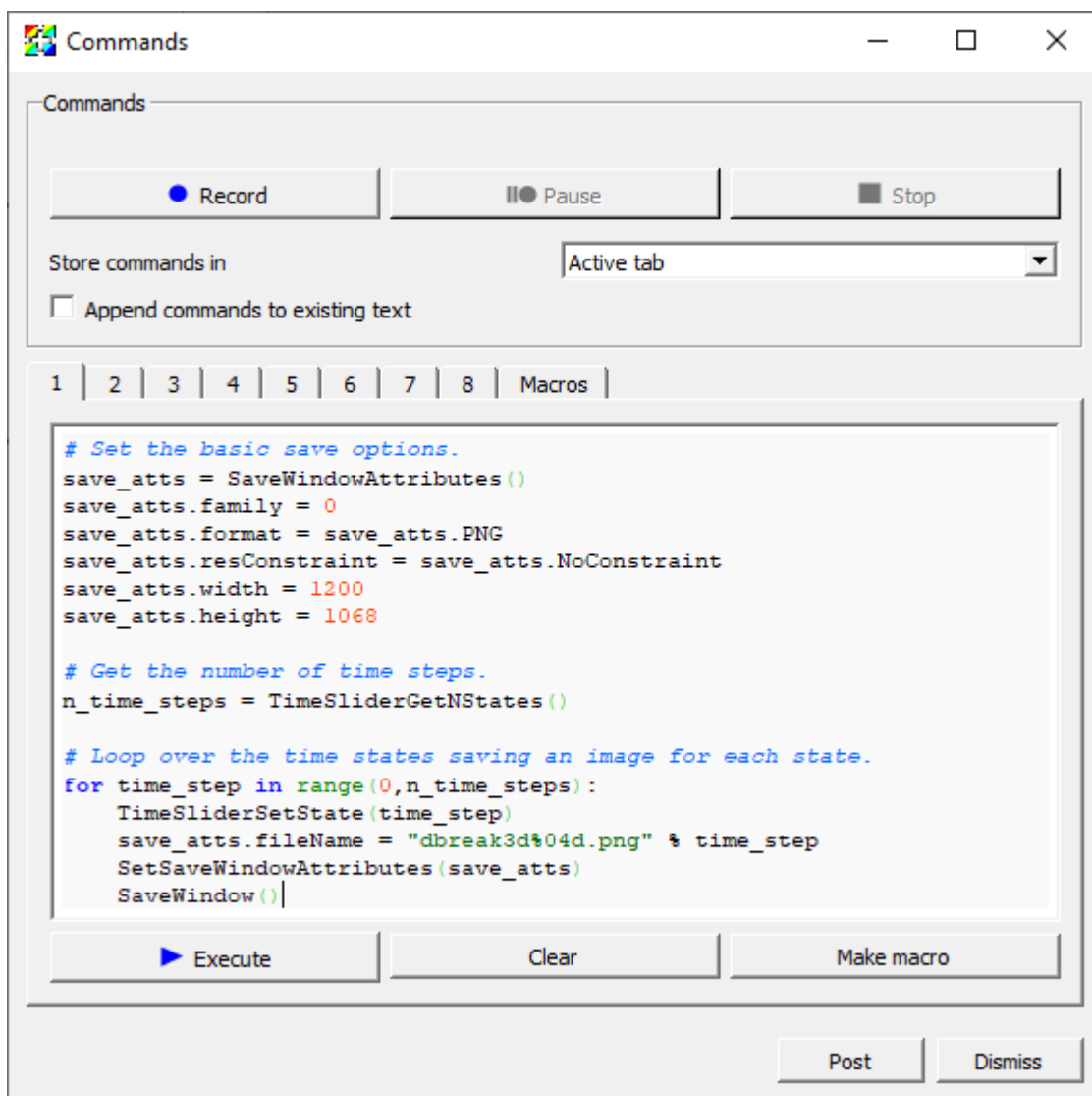
Fig. 3.112: Saving the movie images with a Python script.
