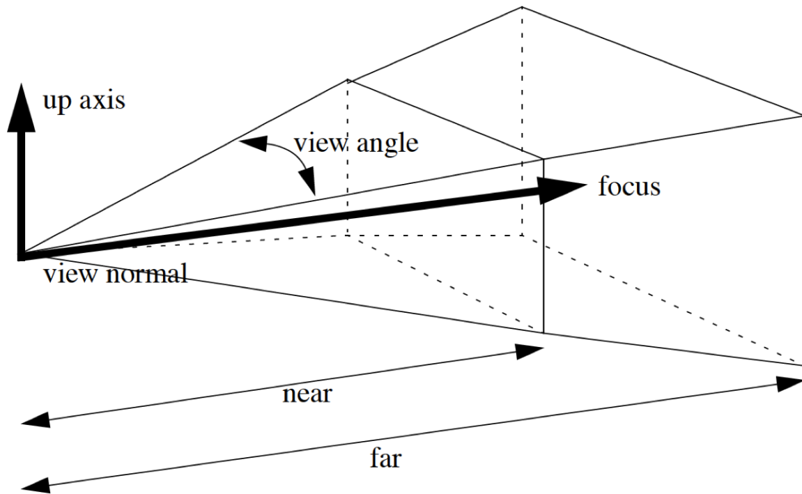
Fig. 1.266: The 3D perspective view volume
