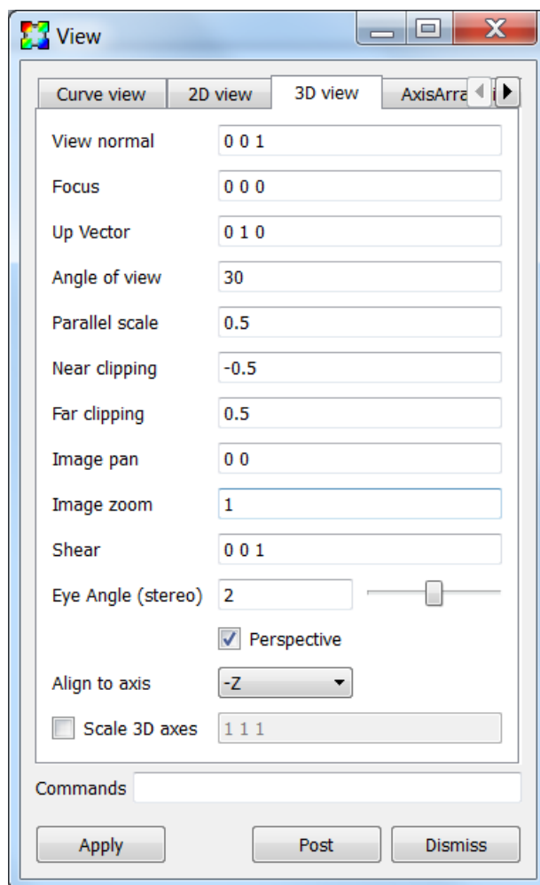
Fig. 1.265: The 3D view options
