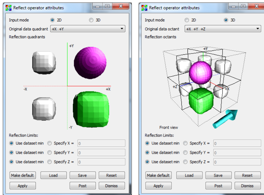
Fig. 1.116: Reflect attributes window
