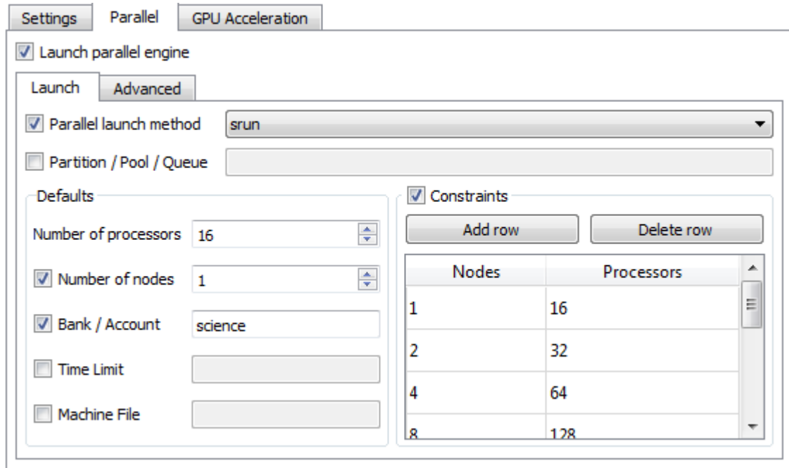
Fig. 1.333: Parallel launch constraints
