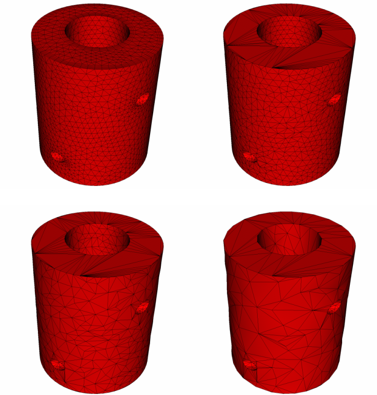
Fig. 1.95: Decimate operator applied to reduce the number of cells in the mesh. (Left-to-right, top-to-bottom): Original Mesh, Reduction = 0.1, Reduction = 0.5, Reduction = 0.75
