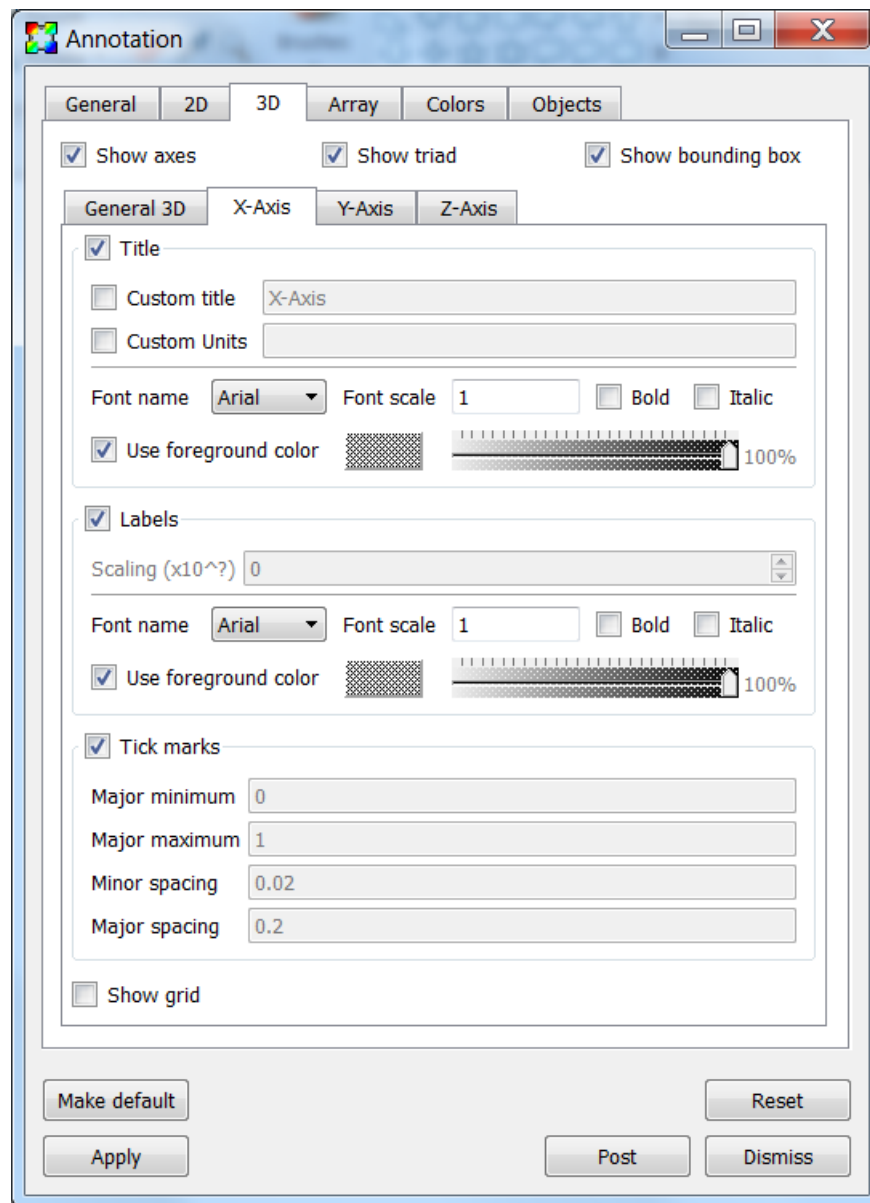
Fig. 1.250: The 3D axes properties
