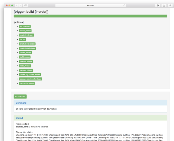
Fig. 1.371: Mansonry Logs in HTML format
