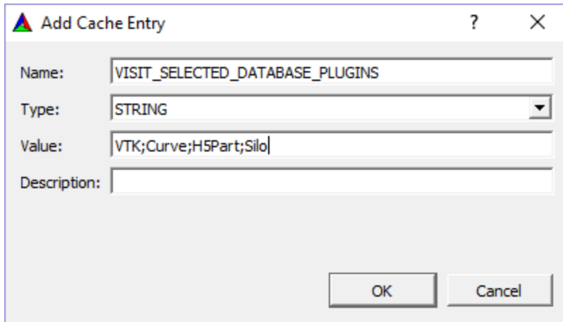
Fig. 1.365: Selecting a limited number of database plugins
