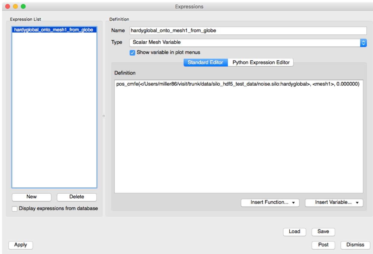
Fig. 1.242: New can be manipulated in the Expression window
