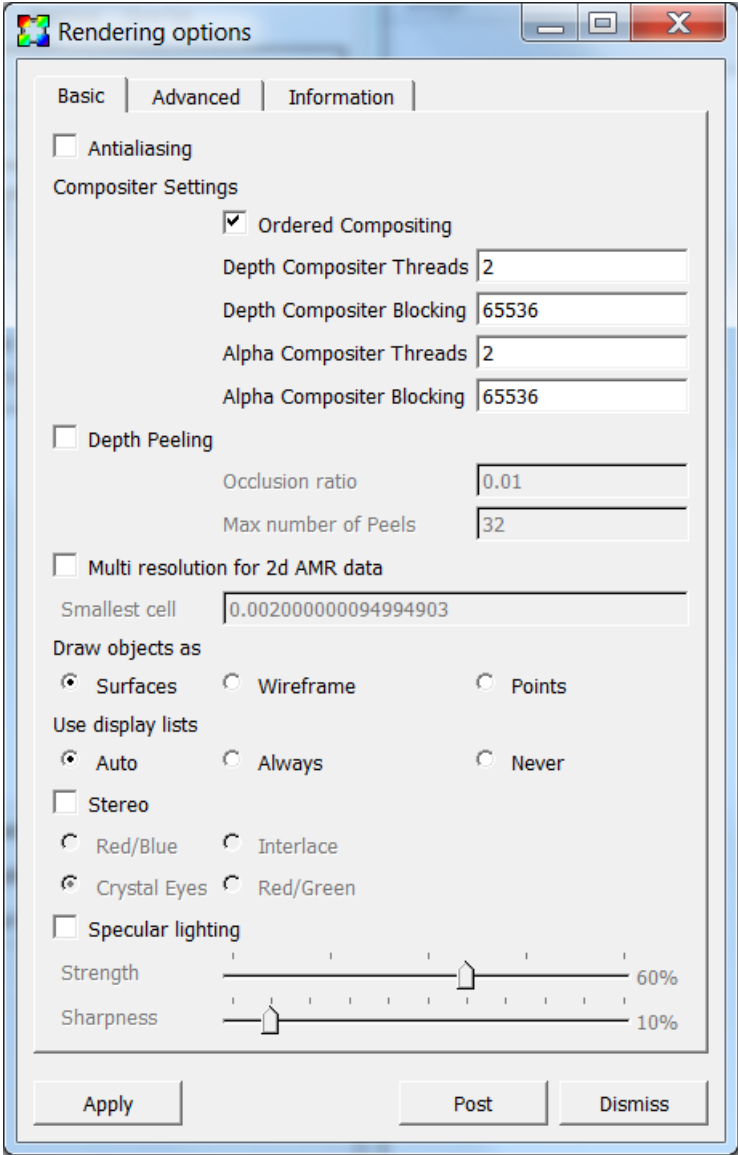
Fig. 1.351: The basic rendering options
