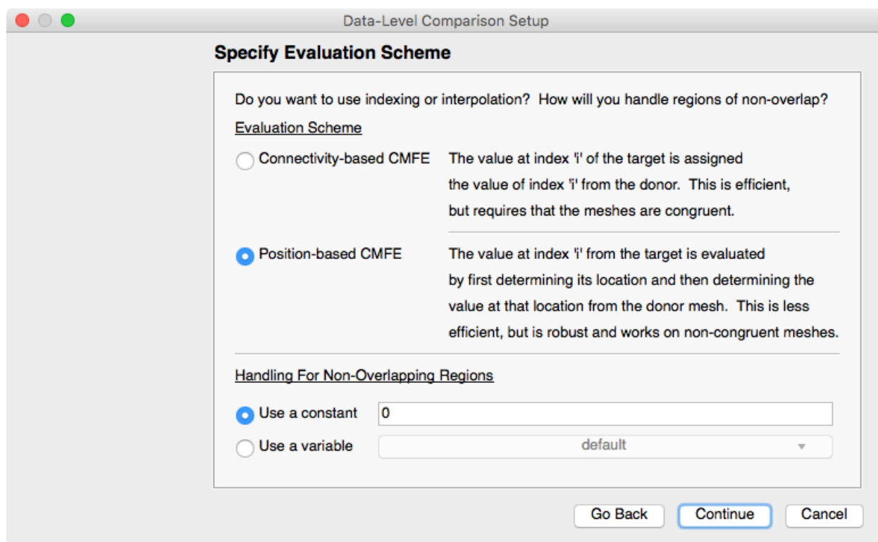
Fig. 1.240: Selecting the mode of evaluation
