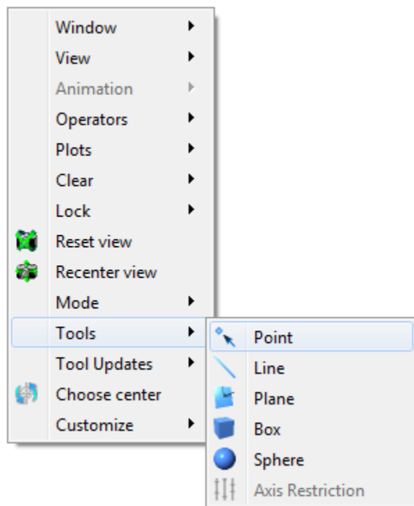
Fig. 1.295: Tools menu
