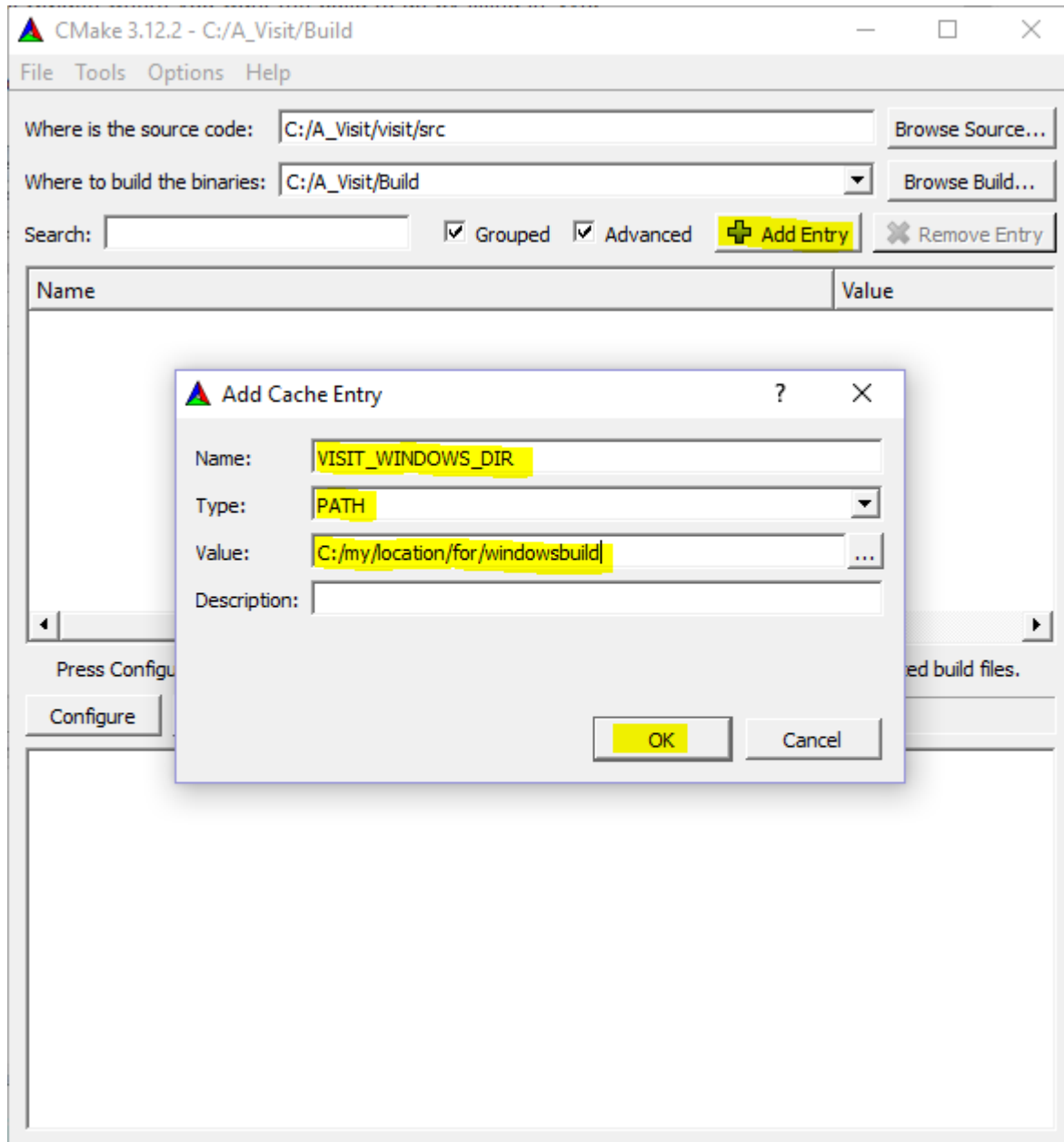
Fig. 1.364: Setting VISIT_WINDOWS_DIR
