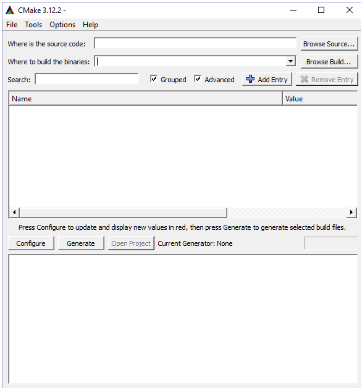
Fig. 1.360: CMake-gui
