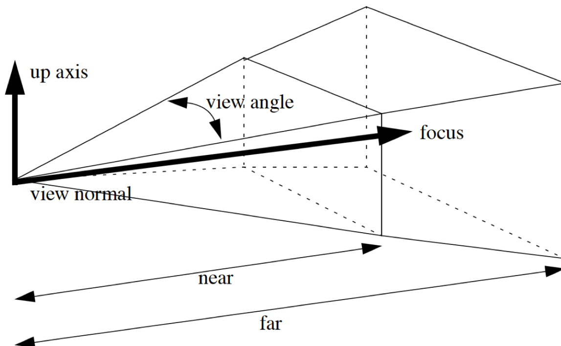
Fig. 1.286: The 3D perspective view volume
