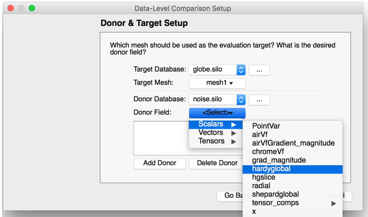
Fig. 1.239: Selecting a specific variable from a database
