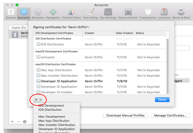
Fig. 1.370: Xcode Manage Certificates Dialog
