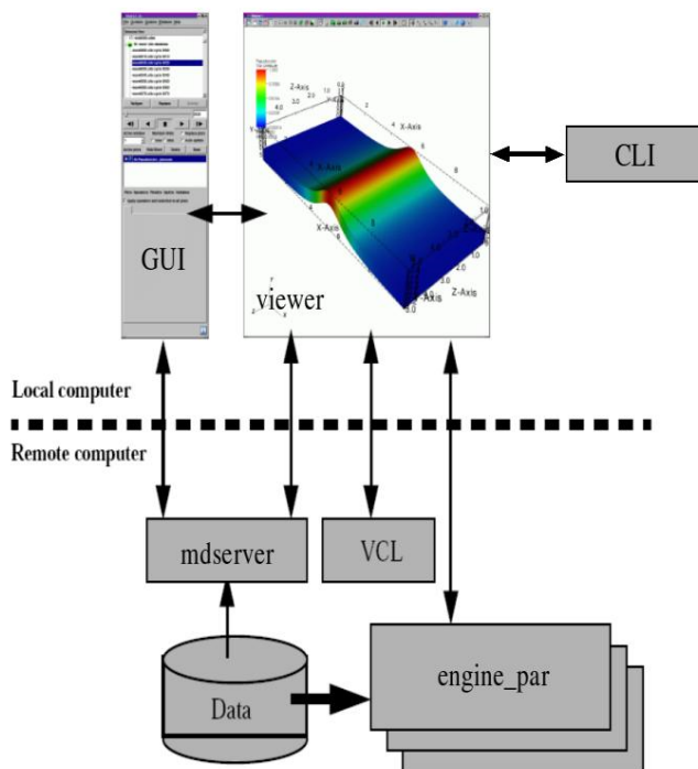
Fig. 1.324: VisIt's Architecture
