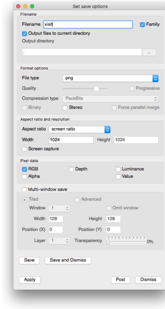
Fig. 1.151: Save Window
