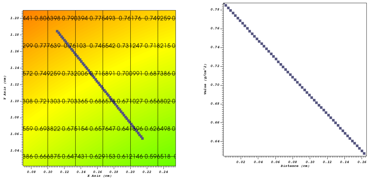
Fig. 1.228: A nodal variable with many sample points.
