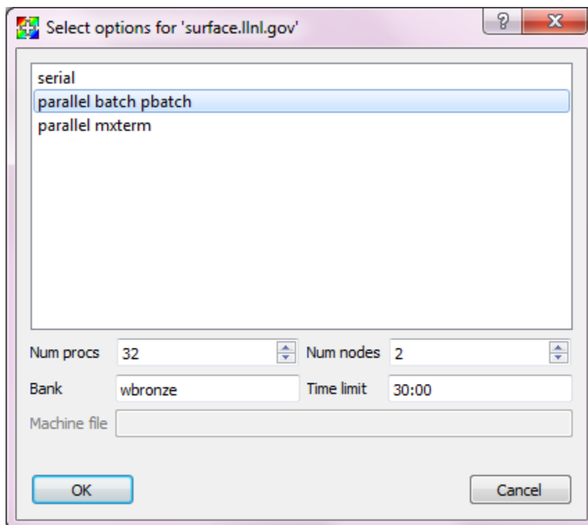
Fig. 1.339: Engine launch options window
