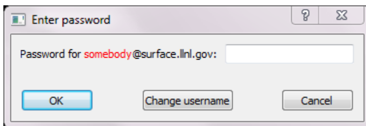
Fig. 1.325: Password Window
