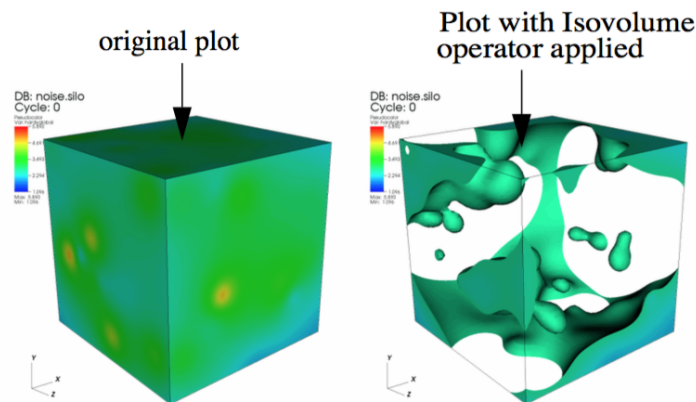
Fig. 2.114: Isovolume Operator Example
