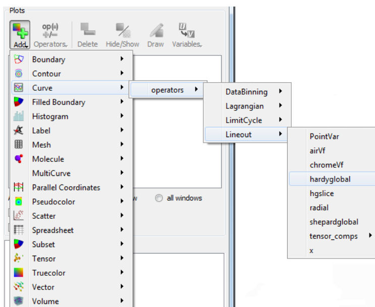
Fig. 2.233: Choosing lineout from the Curve plot's variable menu
