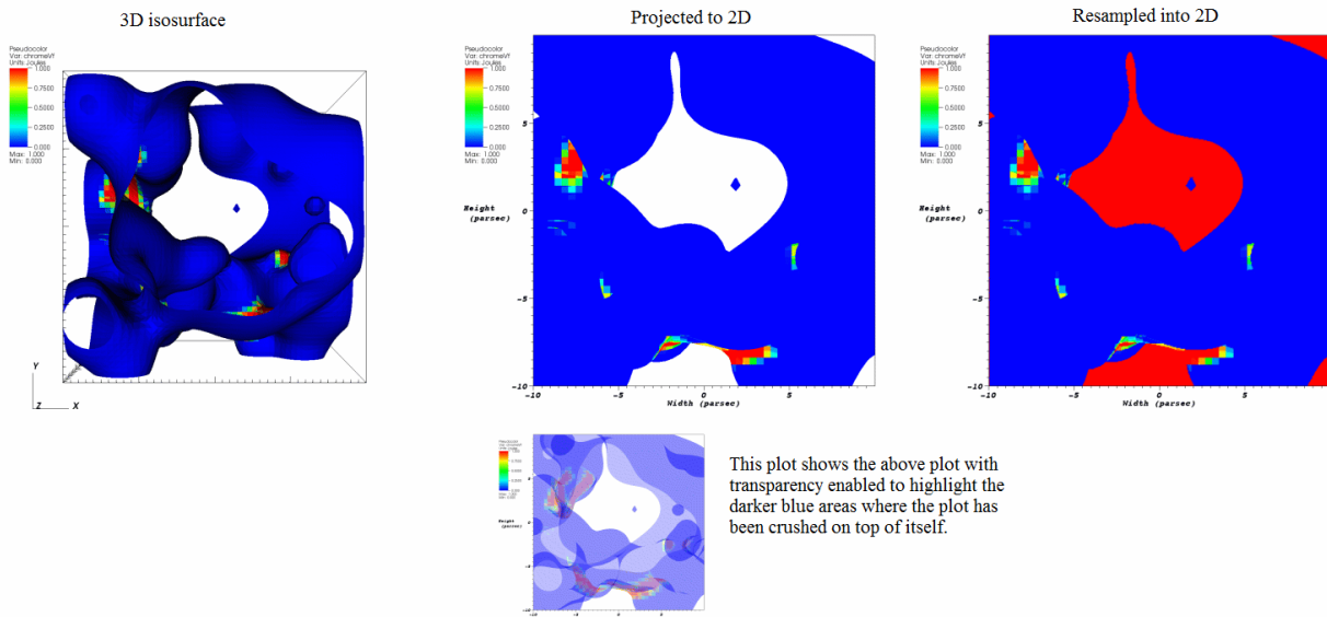
Fig. 2.126: Using the Resample operator to create a 2D projection
