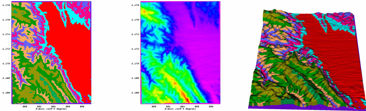
Fig. 2.101: Elevate operator example: 2D plot of rainfall; 2D plot of elevation; Plot of rainfall elevated by elevation
