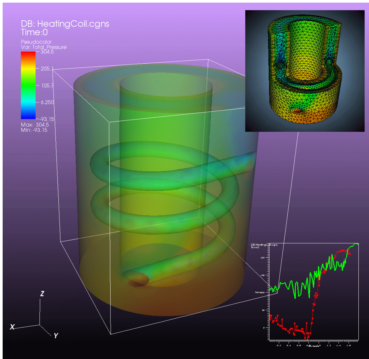
Fig. 2.266: An Example of a visualization with two overlaid image annotations
