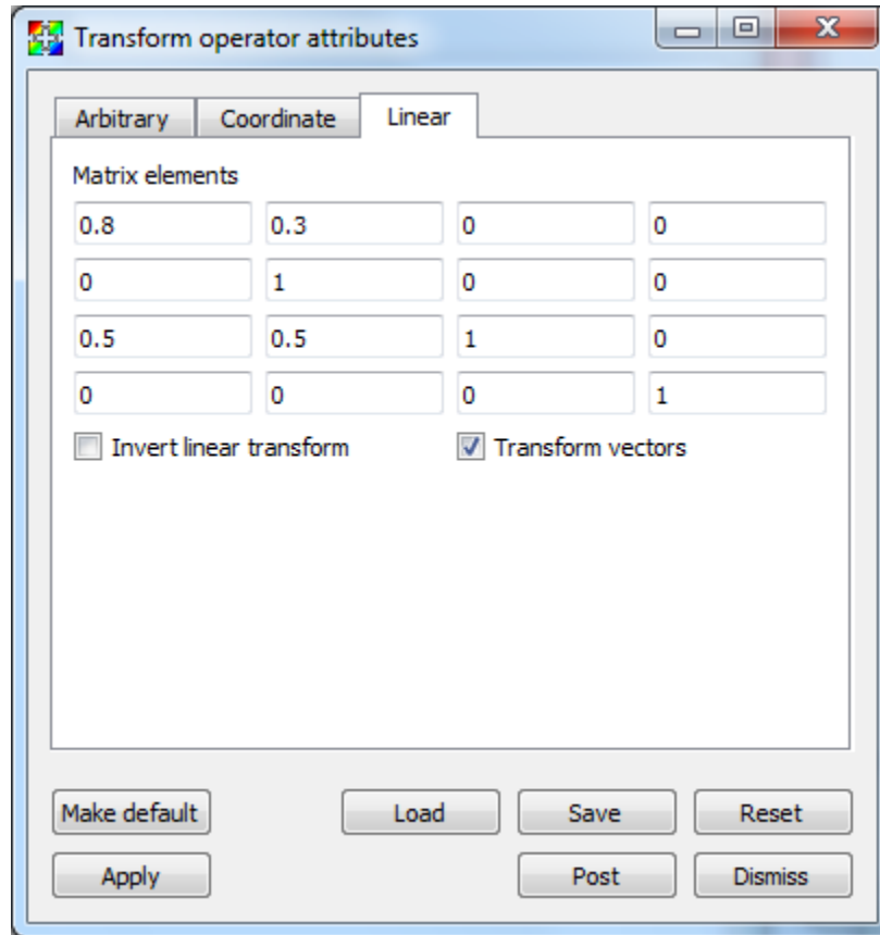
Fig. 2.148: Linear transformation options
