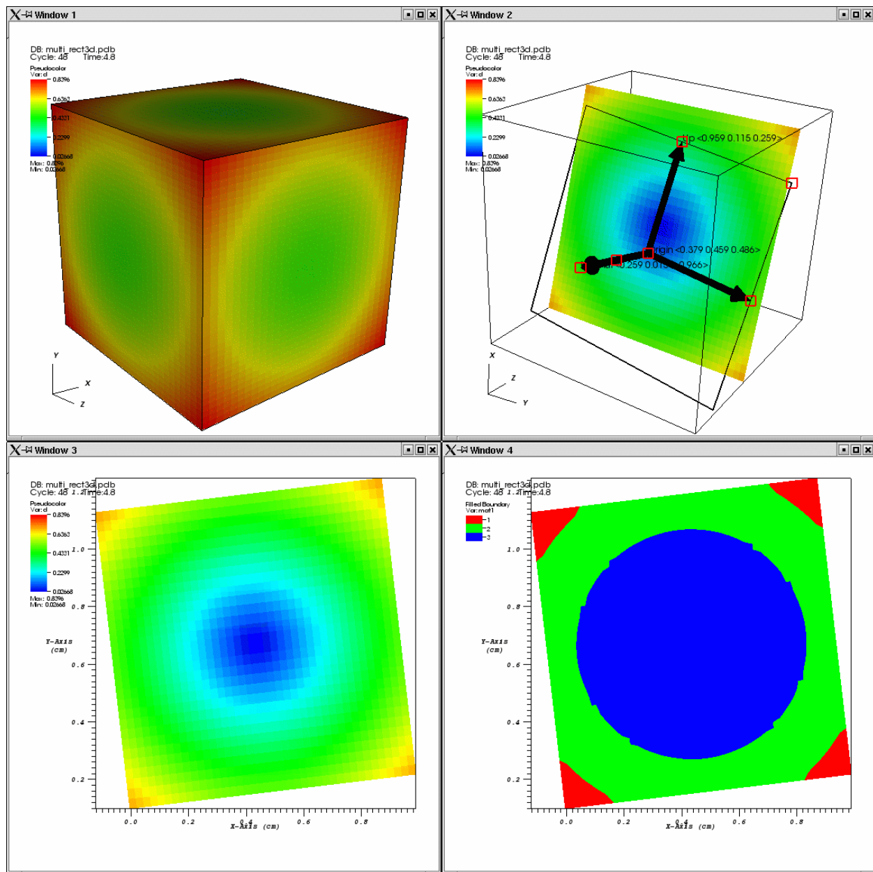
Fig. 2.324: Multiple visualization windows with locked tools
