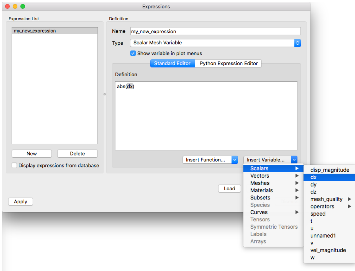
Fig. 2.207: Expression Window's Insert Variable... menu
