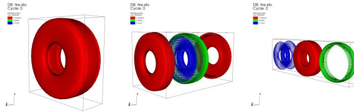
Fig. 2.105: Explode operator example: original plot; exploding cells of a material; exploding materials.
