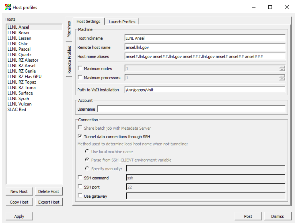
Fig. 4.129: The Host profiles window with the host profiles for LLNL
