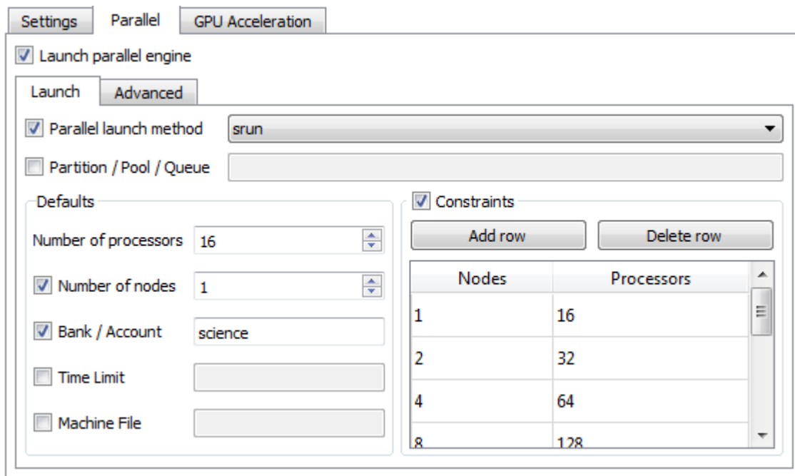
Fig. 2.334: Parallel launch constraints
