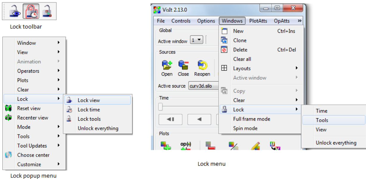
Fig. 2.323: Mechanisms for locking windows
