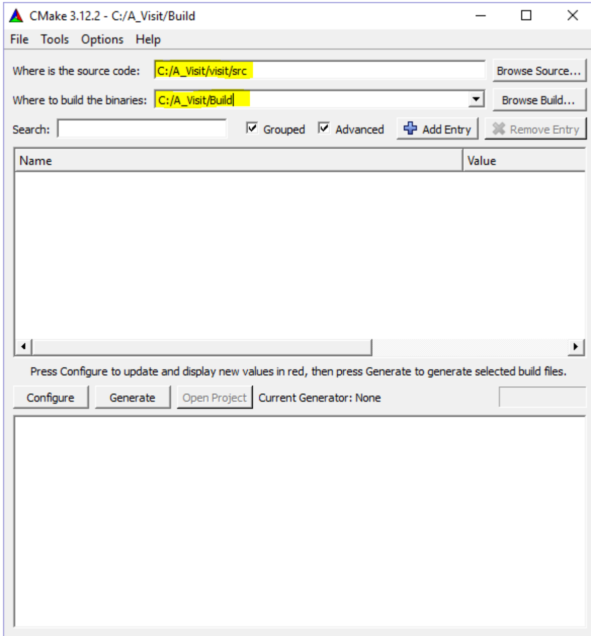
Fig. 2.362: Setting source and build directories
