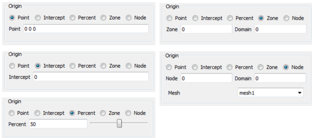
Fig. 2.131: Origin area appearance
