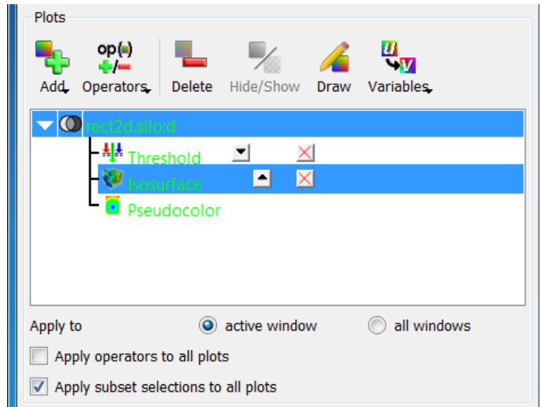
Fig. 2.79: After removing an operator from the middle of the pipeline
