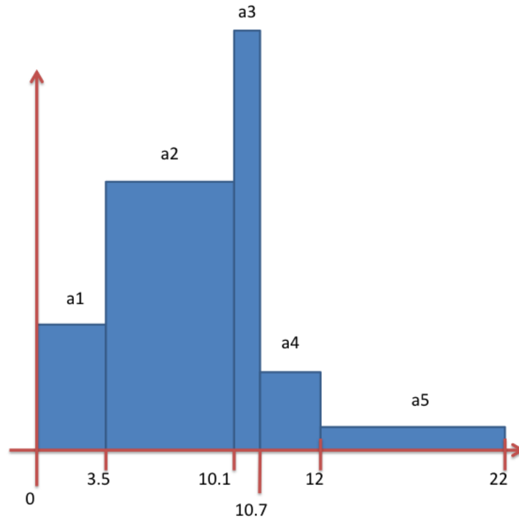
Fig. 2.208: Bar graph created from picking an array variable created with array_compose_with_bins()
