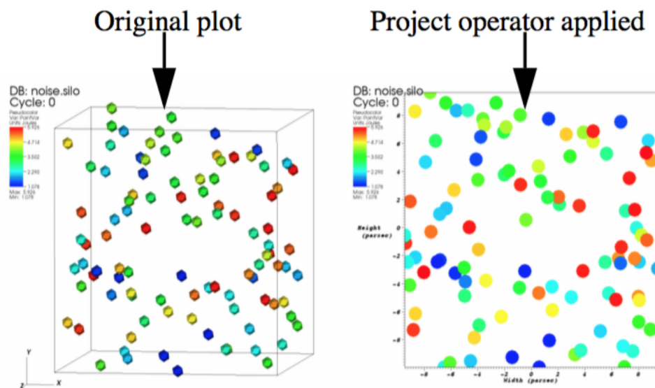
Fig. 2.118: Project Operator Example
