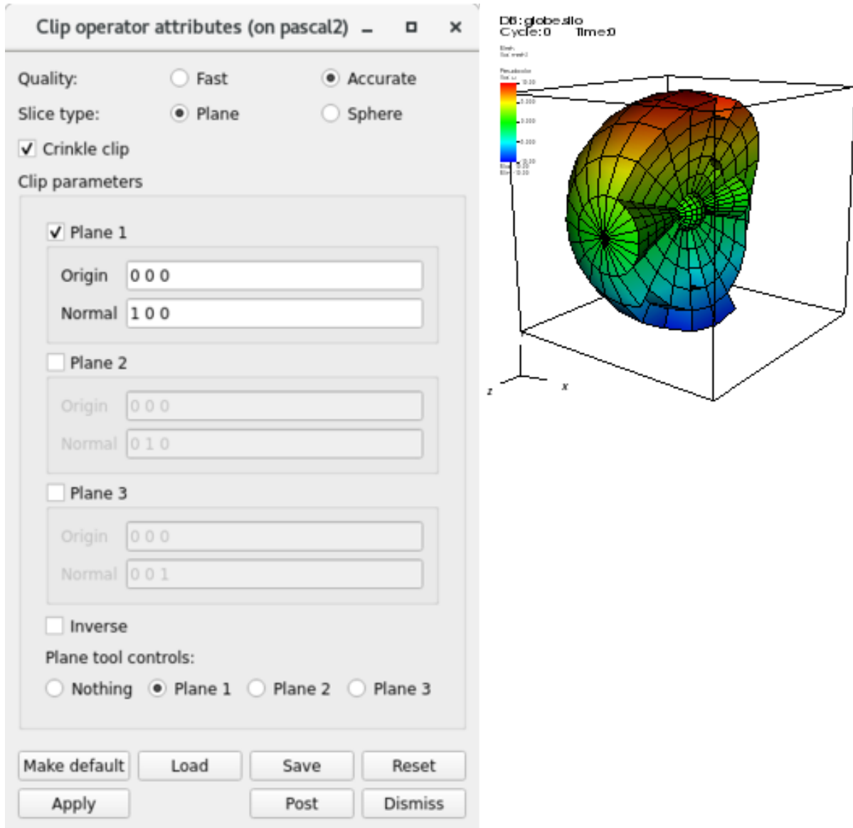
Fig. 2.88: Enabling the Crinkle clip option; Crinkle clip example
