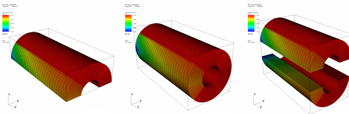
Fig. 2.121: Reflect operator example
