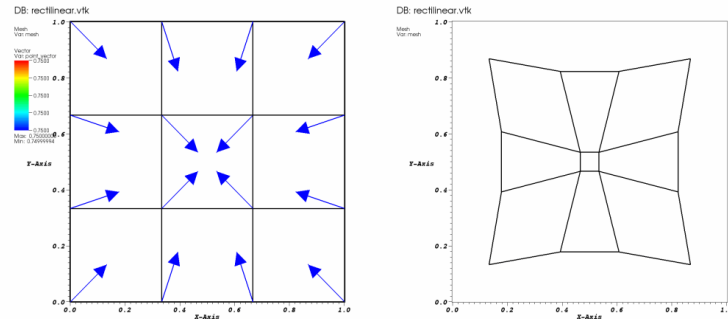
Fig. 2.99: Mesh and Vector plots and a Mesh plot that uses the Displace operator to deform the mesh using a vector field.
