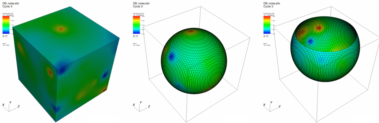
Fig. 2.134: SphereSlice operator example
