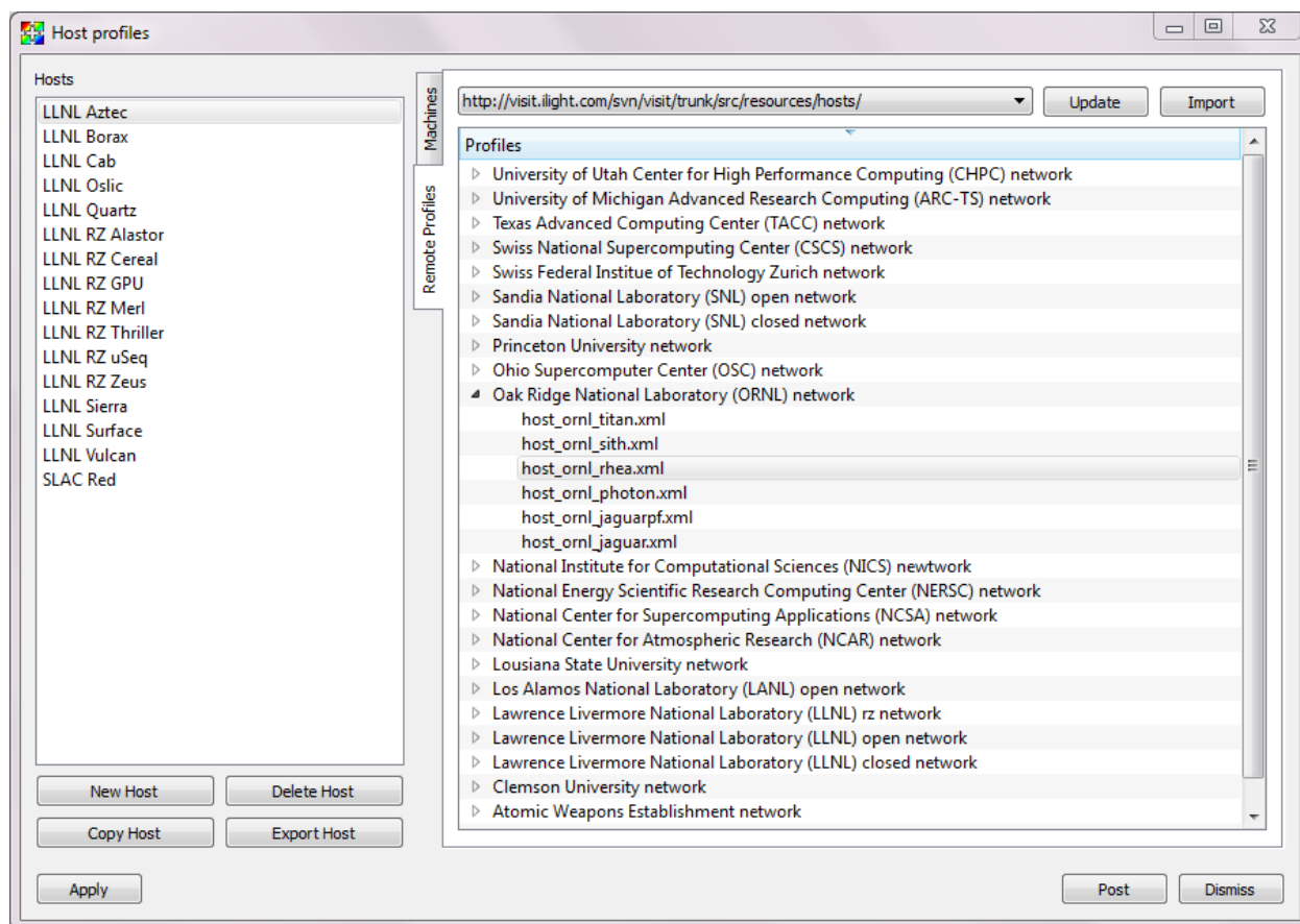
Fig. 2.339: Remote Profiles tab with host selected for import
