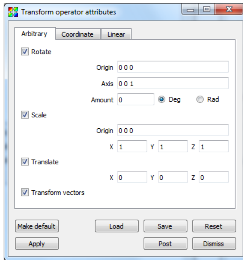
Fig. 2.144: Transform attributes window
