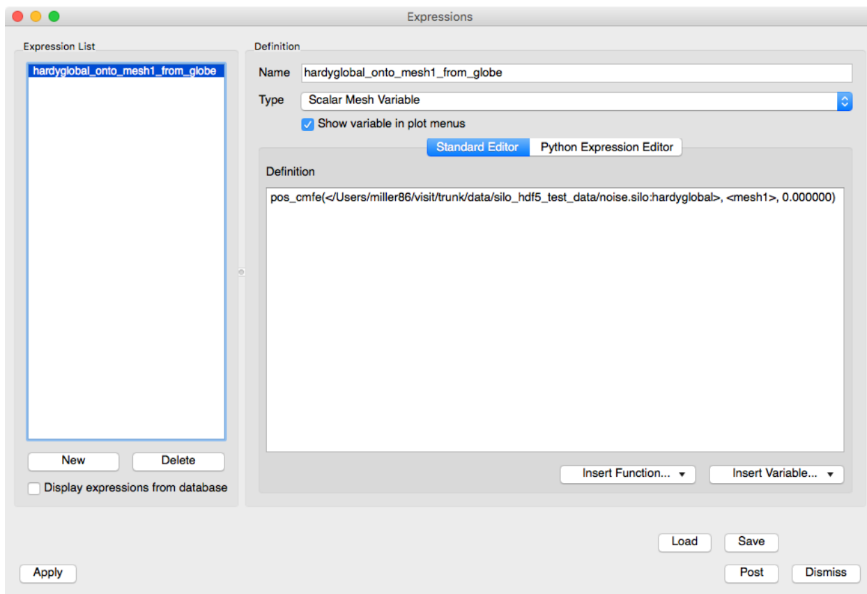
Fig. 2.243: New can be manipulated in the Expression window
