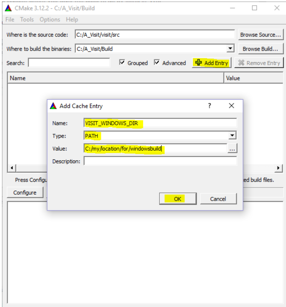
Fig. 2.374: Setting VISIT_WINDOWS_DIR
