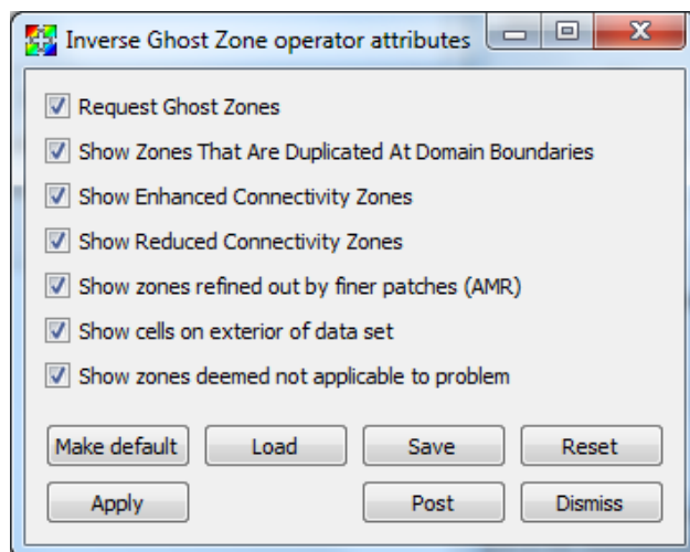
Fig. 2.119: InversetGhostZone window
