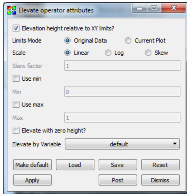
Fig. 2.110: Elevate window
