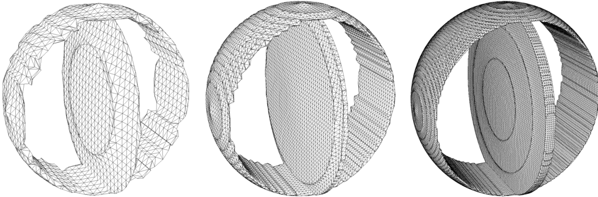
Fig. 2.134: The Resample operator can be used to control the resolution of CSG meshes. Resolution is increased from left to right.
