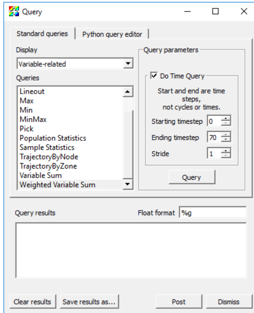
Fig. 4.12: The Weighted Variable Sum query
