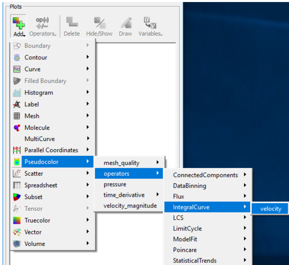
Fig. 4.43: Creating a streamline plot with the IntegralCurve operator.
