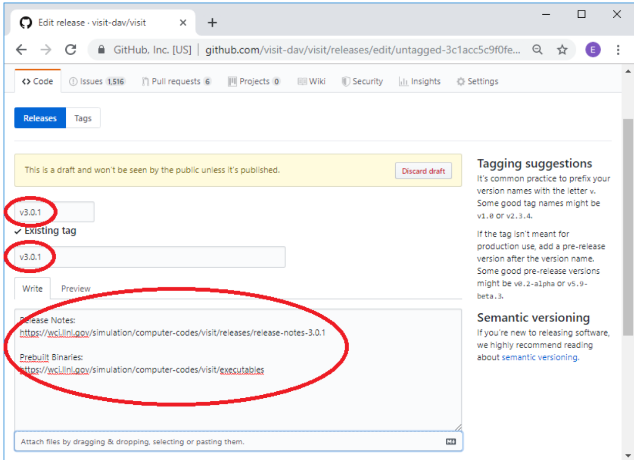
Fig. 5.9: Entering information about the release.
