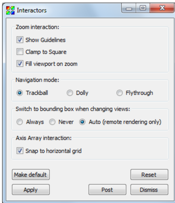
Fig. 2.187: Interactors window
