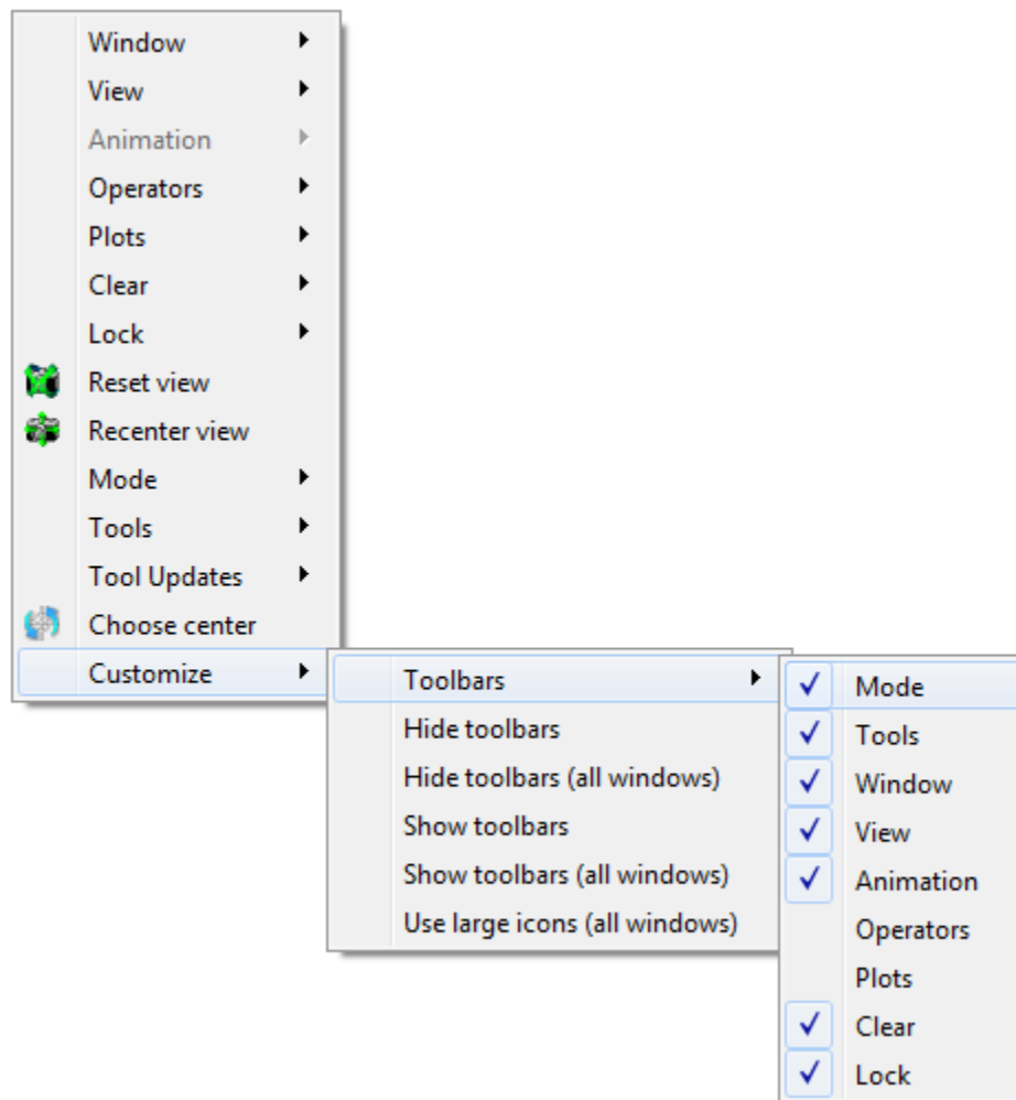
Fig. 2.188: Customize menu
