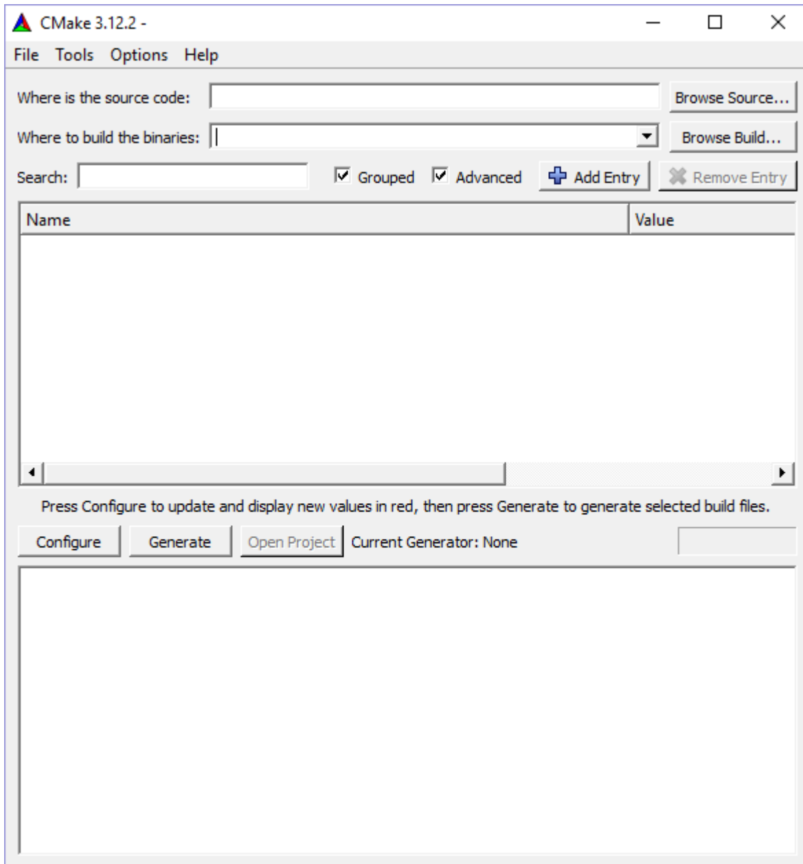
Fig. 2.370: CMake-gui
