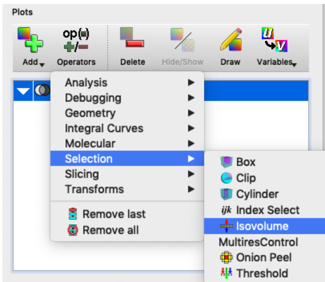
Fig. 4.77: Adding a Isovolume operator.
