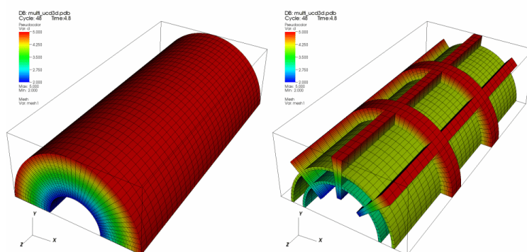
Fig. 2.118: InversetGhostZone example
