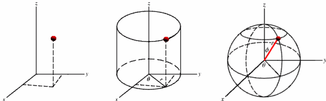
Fig. 2.154: Cartesian, Cylindrical, Spherical coordinate systems
