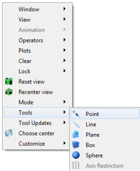
Fig. 2.305: Tools menu
