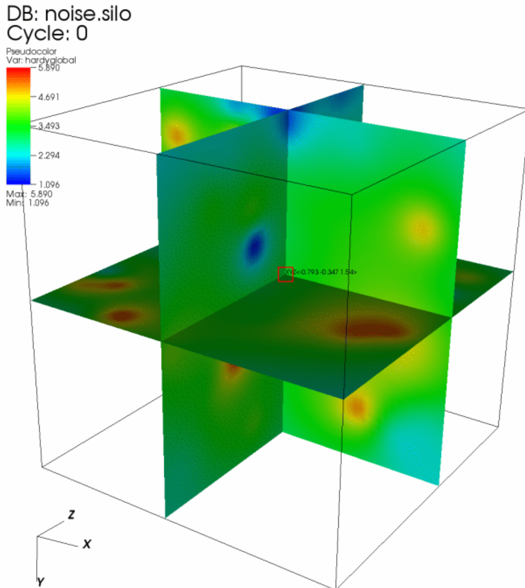
Fig. 2.311: Point tool
