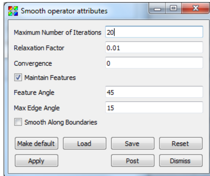
Fig. 2.142: Smooth attributes
