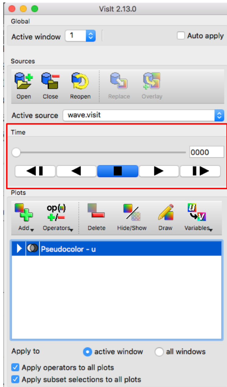
Fig. 2.300: Animation controls
