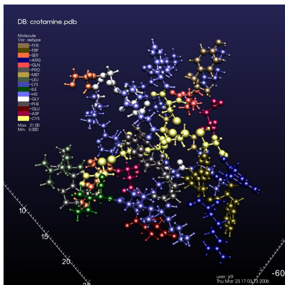
Fig. 2.50: Molecule plot of croptamine, colored by residue type, atoms proportional to covalent radius emulating the CPK style, bonds colored with adjacent atom color.
