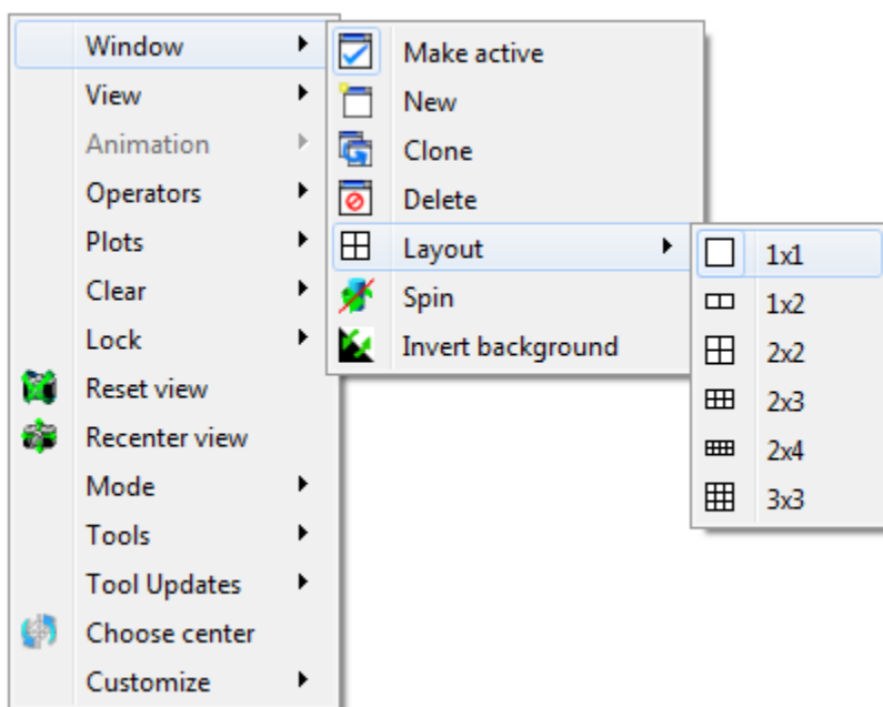
Fig. 2.180: Window menu
