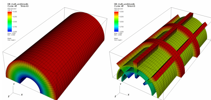
Fig. 4.122: InversetGhostZone example
