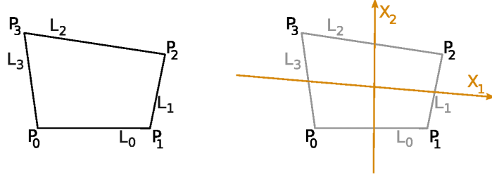
(a) Vertices of a quadrilateral.
